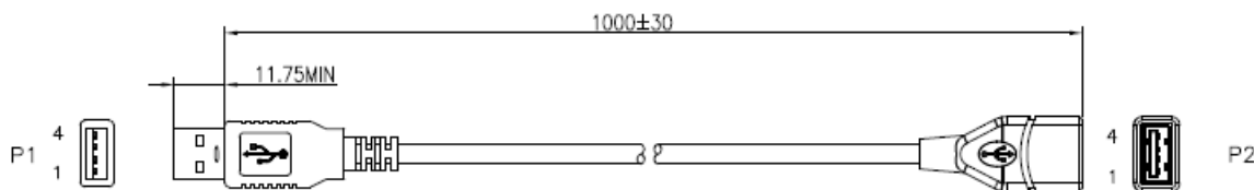
Outline Drawing
